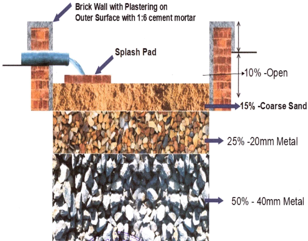
Rain water Harvester pit diagram
